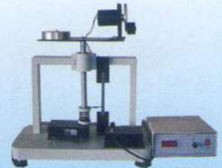
TRANSMISSIBILITY RATIO
