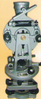
Vernier Transit Theodolite
